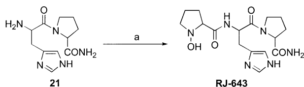
Scheme 2. (a) N -hydroxy-L-Pro-OH, DCC, HOBT, DMF.
