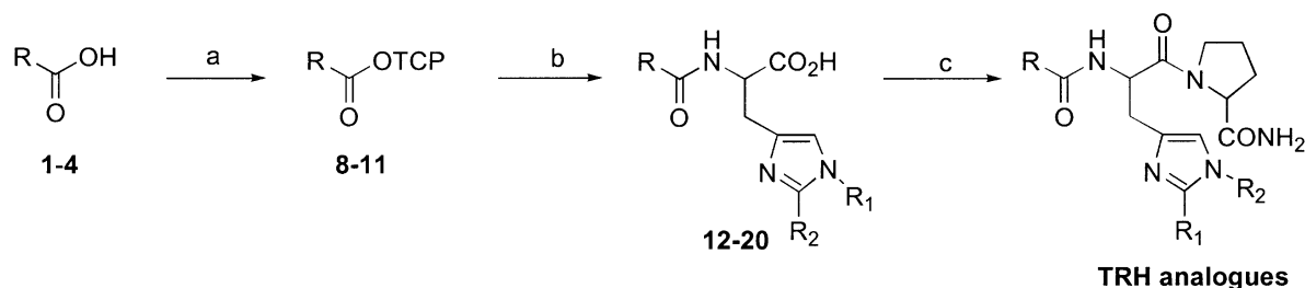
Scheme 1. (a) 2,4,5-trichlorophenol, DCC, DMF; (b) i. H-His(R 1 ,R 2 )-OMe, EtOAc; ii. 0.5 N NaOH, MeOH, ion-exchange (H + ); (c) Pro-NH 2 , DCC, HOBT, DMF.
